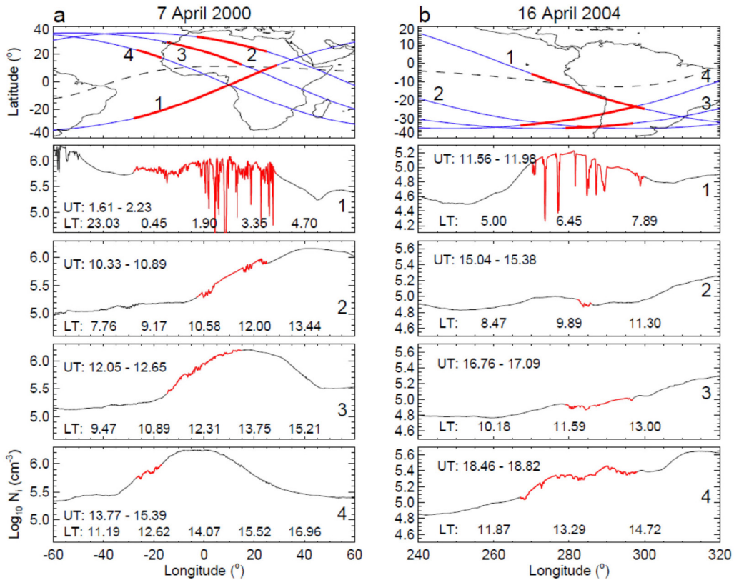
Fig. 6. Tracing of the history of daytime irregularities shown in the ROCSAT-1 observations. Adapted from Kil et al. (2019) with CC-BY. In the ROCSAT-1 orbits and density data (orbits 2–4), the locations of daytime irregularities are indicated in red. Orbit 1 for both days is the orbit on the previous night. ROCSAT-1, Republic of China satellite.
